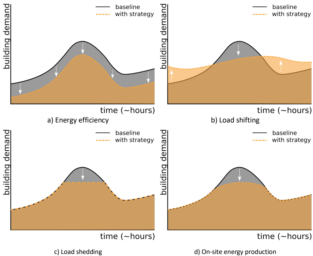
Figure 3: Overview of selected demand side management strategies (reproduced from Fosás et al. 2020).
